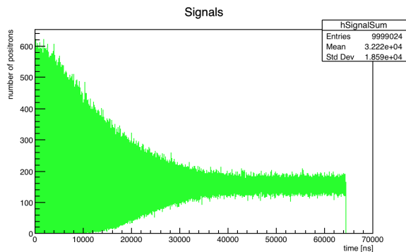
Figure 3: Simulated decay positron signal as a function of time from injection.
