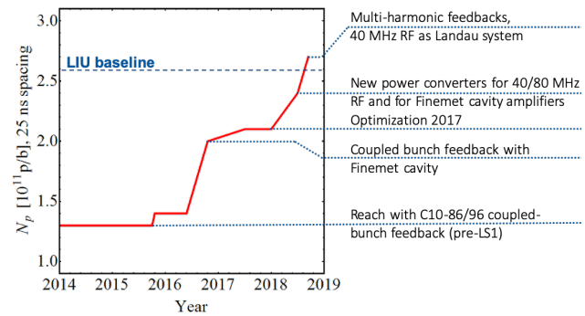
Figure 3: Evolution of bunch intensity in the PS over Run 2.
