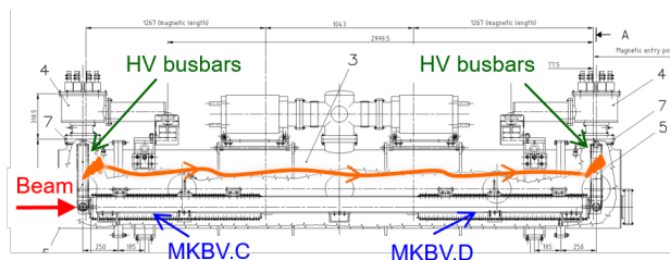
Figure 1: Overview of the two vertical dilution kickers inside their common vacuum tank. The first flashover occurred at the MKBV.C and then propagated downstream to the MKBV.D. The propagation path in orange is indicated for illustration purposes only.
