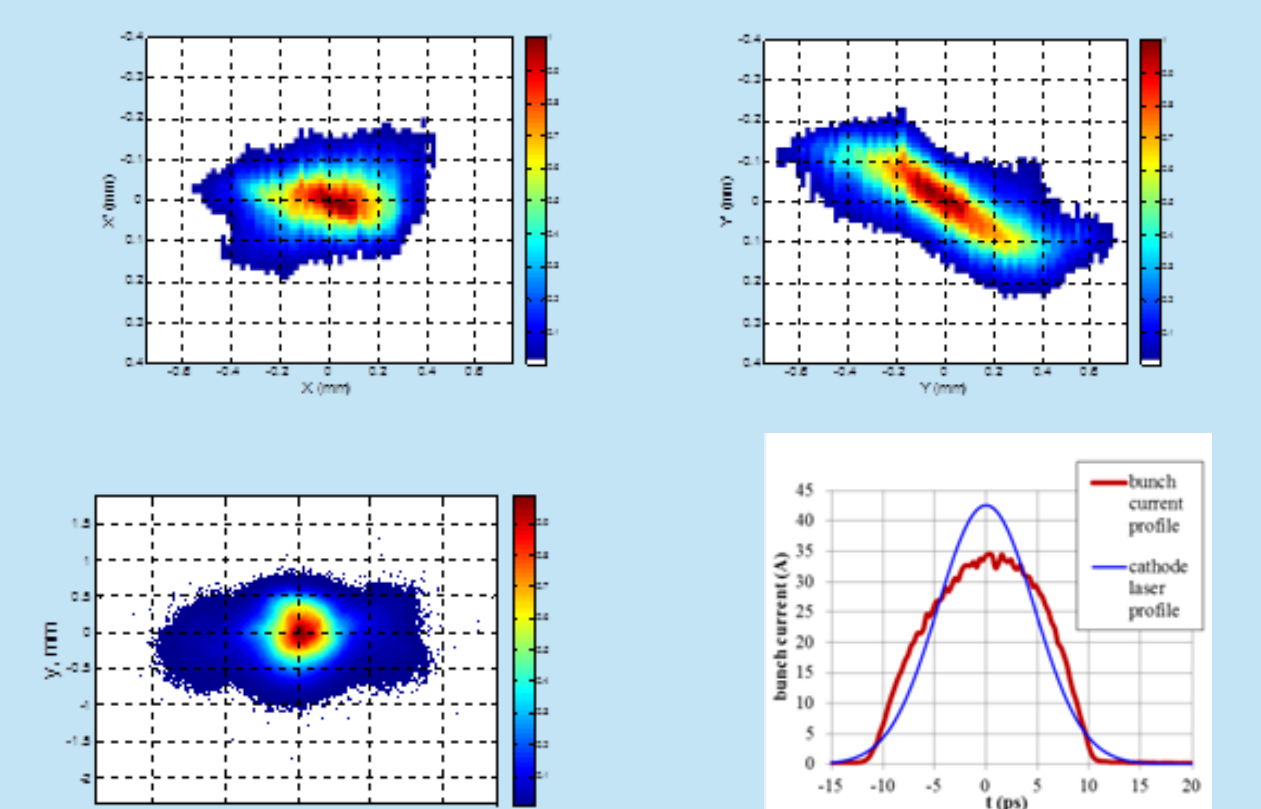
Electron beam transverse distribution at a YAG screen. Bunch current profile was measured using a transverse deflecting system [3].
