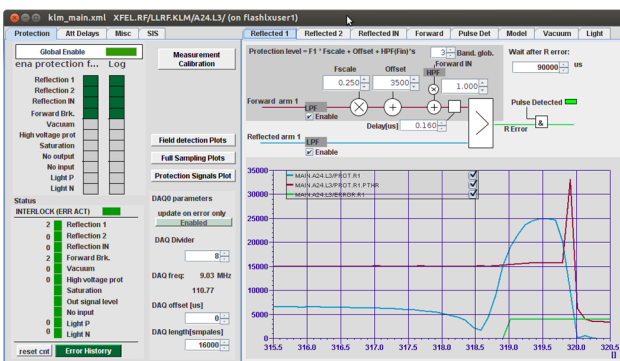
Figure 4: Detection of WG breakdown, A24.L3.
