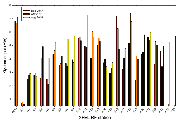
Figure 2: Output power for each of MBK.
