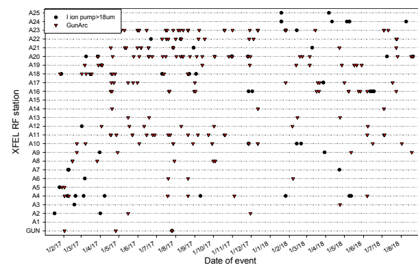
Figure 5: Gun HV arcing and RF breakdowns in XFEL MBKs.
