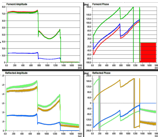
Figure 7: The output RF shapes of MBK in case of using phase modulation.
