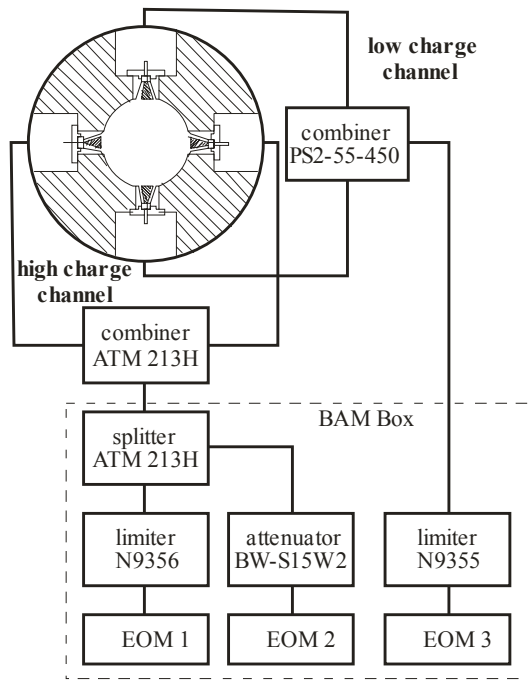
Figure 2: Proposed cabling plan and components for the 40 GHz BAM.
