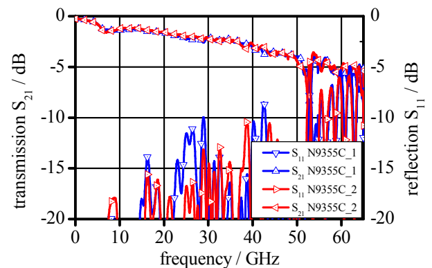
Figure 4: Transmission coefficient for the limiters Agilent N9355C.
