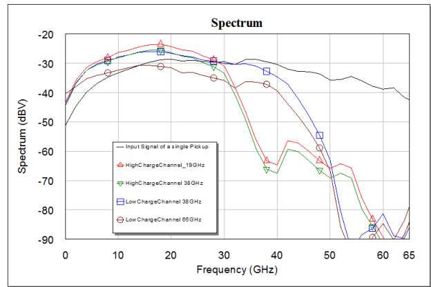
Figure 12: Simulated spectrum of the low and high charge channel.
