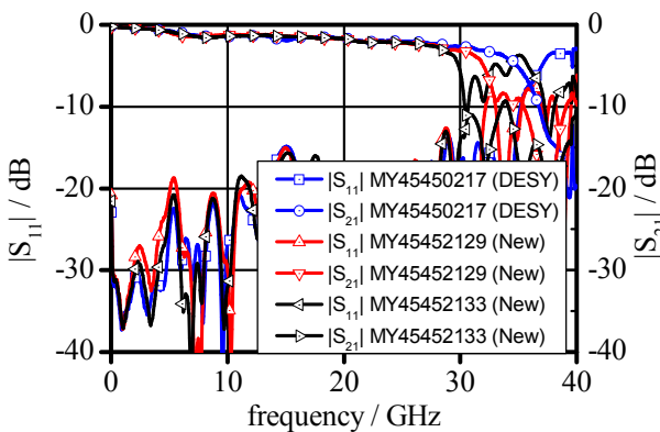
Figure 6: Transmission coefficient for Agilent N9356 limiters.
