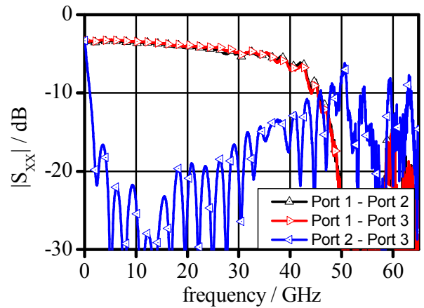
Figure 3: Transmission and reflection coefficient versus frequency of the RF-combiner PS2-55-450.
