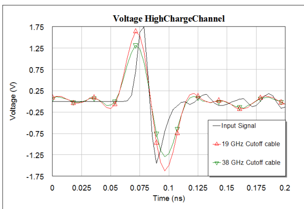
Figure 9: Voltage response of the high charge channel for different cable types for a bunch charge of 20pC.
