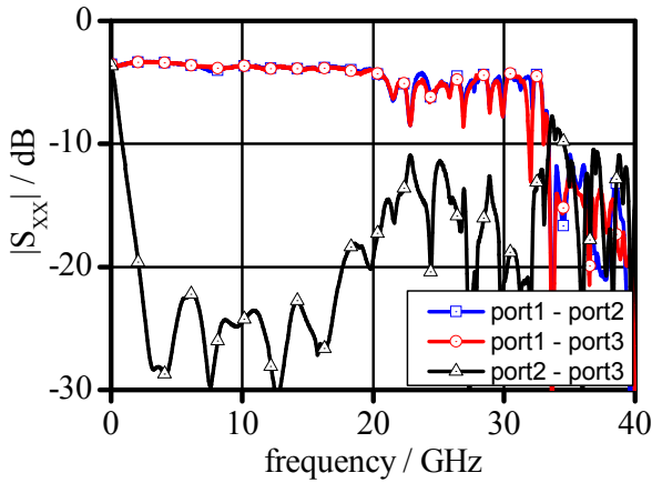
Figure 5: Transmission coefficient of the combiner ATM 213H.
