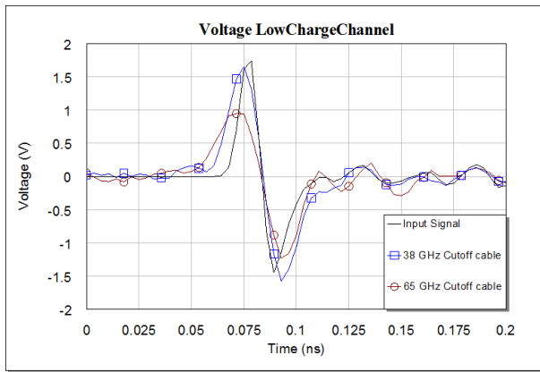
Figure 11: Simulated voltage response of the low charge channel for 3.58 mm cables and 2.286 mm cables for a bunch charge of 20pC.
