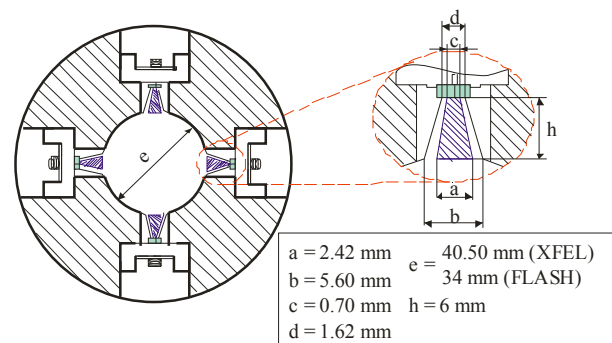
Figure 1: Cross-section of the cone-shaped pickup [5].
