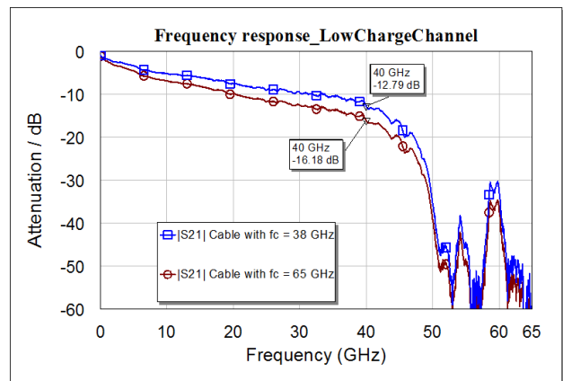
Figure 10: Simulated frequency response of the low charge channel for 3.58 mm cables and 2.286 mm cables.
