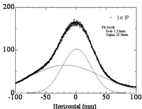
Figure 9: Beam profile in horizontal direction obtained by the IP with fitting of two Gaussian curves.
