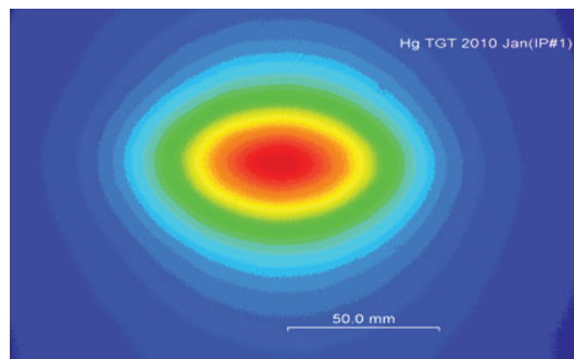
Figure 8: Two dimensional beam profile obtained by the IP attached to the target vessel.
