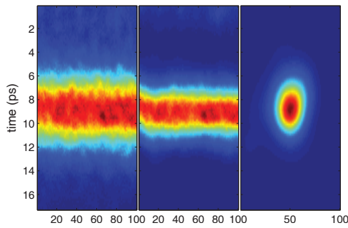
Figure 4: SC images: Left, raw image with \alpha \approx 1.210^{-6} ; Middle, same image but deconvolved; Right, SC PSF. Horizontal axis represents the slow axis sweep set to 500 \mu\text{s}/\text{mm} . On each image a region of interest of 100 \times 100 pixels is selected, equivalent to \approx 17 ps \times 600 \mu\text{s} .
