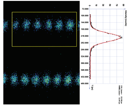
Figure 8: Example of a bunch length measurement.
