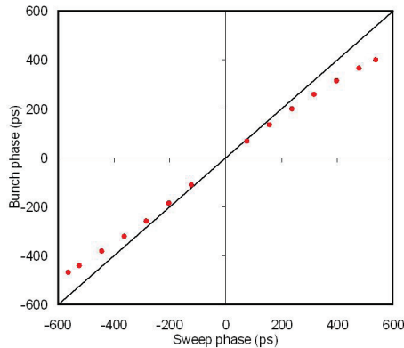
Figure 3: Linearity using the 50ps/mm sweep speed.
