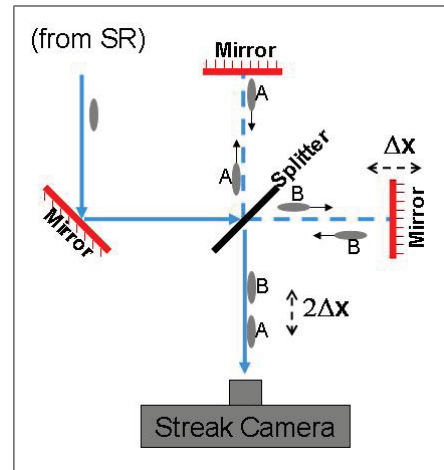
Figure 4: Calibration set-up.
