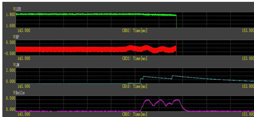
Figure 2: Examples of logged signals at a moment of (a) a manual beam abort, (b) a beam phase abort caused by RF voltage down and (c) a beam loss abort caused by vacuum problem. Signals in (c) are the LER beam current, the beam phase, the loss monitor PD and the Belle PD from top to bottom.
