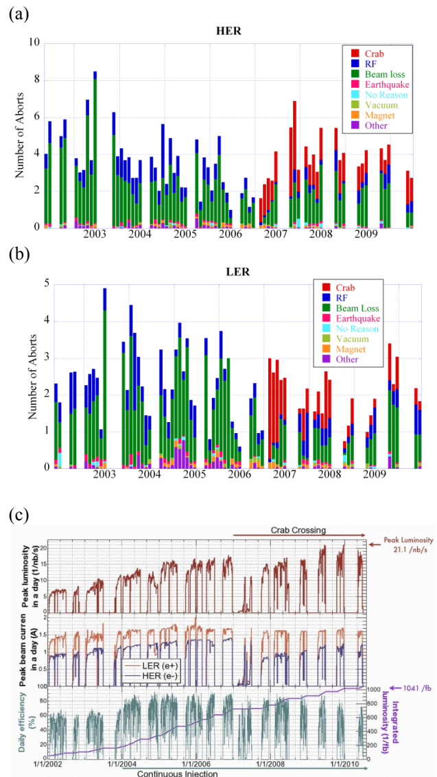
Figure 5: Statistics of the beam abort for last eight years of KEKB operation in HER (a) and LER (b). (c) History of the beam current and the luminosity of KEKB.
