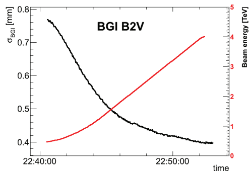
Figure 4: Beam size behaviour during ramp of Pb beam. Beam energy is given in ZTeV.
