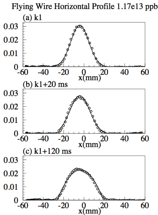
Figure 4: Horizontal beam profiles at the trigger of k1 (a), k1+20 ms (b), k1+120ms (c).
