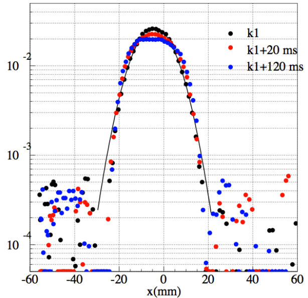
Figure 3: Horizontal beam profiles of the two-bunch beam for the intensity of 0.95 \times 10^{13} ppb. The beam profile at the injection timing k_1 is shown in black circles and the fitted Gaussian function is shown in the solid line. Profiles at 20 ms after the injection and at 120 ms after the injection are shown in red circles and blue circles respectively.
