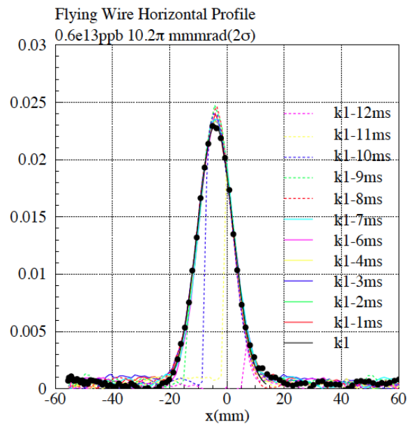
Figure 6: Horizontal beam profiles at the injection for the beam intensity of 0.6 \times 10^{13} ppb.
