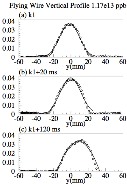
Figure 5: Vertical beam profiles at the trigger of k1 (a), k1+20 ms (b), k1+120ms (c).
