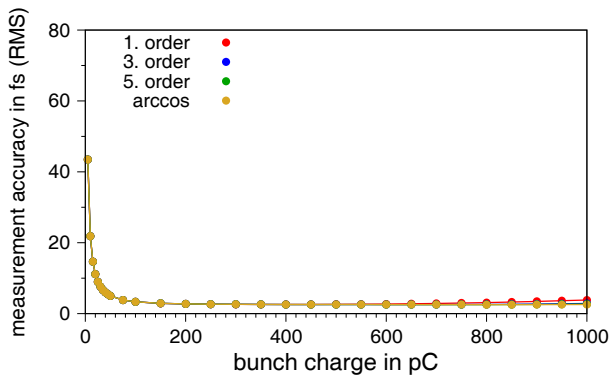
Figure 5: Calculated measurement accuracy of the BAM system at the 40 GHz EOM for different bunch charges with a timing jitter of 25 fs.
