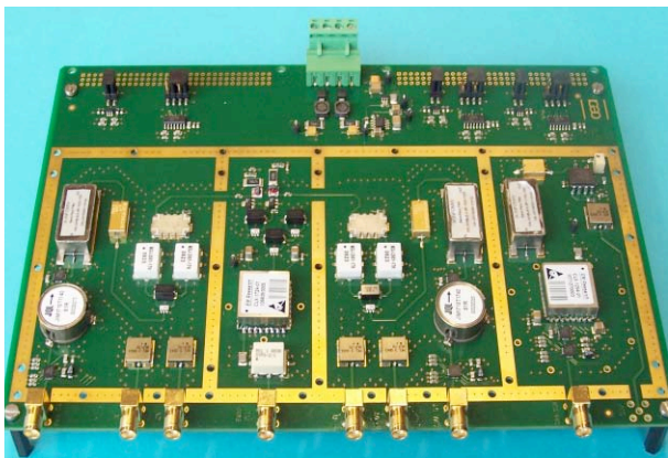
Figure 5: Re-entrant RFFE board.
