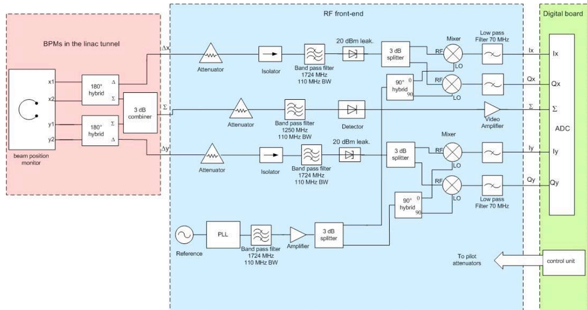
Figure 4: RF signal processing electronics.
