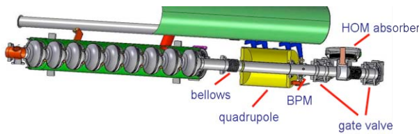
Figure 2: Layout of the downstream end of the XFEL cryomodule.
