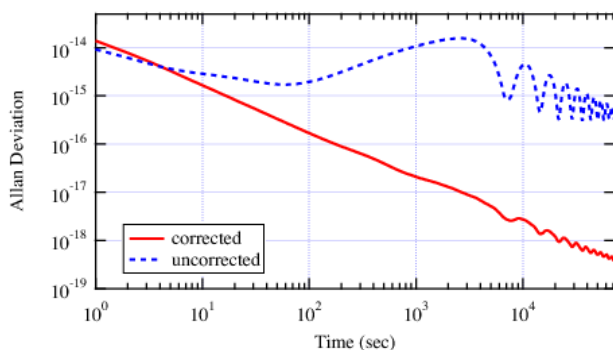
Figure 4: Allan deviation of the relative timing of a 2 m and a 2.2 km link. Dotted line: uncorrected RF delay. Solid line: corrected RF delay.
