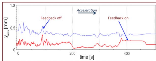
Figure 3: Comparison of vertical orbit rms, measured in Blue ring on two consecutive ramps. The orbit rms on the ramp without feedback affected by the diurnal orbit variations. The ramp with the feedback on produces considerably improved orbit.
