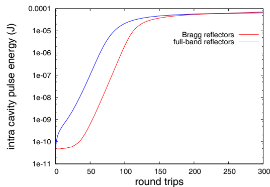
Figure 2: FEL pulse evolution for two types of optical cavities with Bragg reflectors and full-band virtual reflectors
