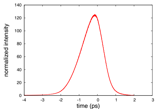
Figure 6: Temporal profile of a saturated FEL pulse with Bragg reflectors. ( dL = -5.6\mu\text{m} )
