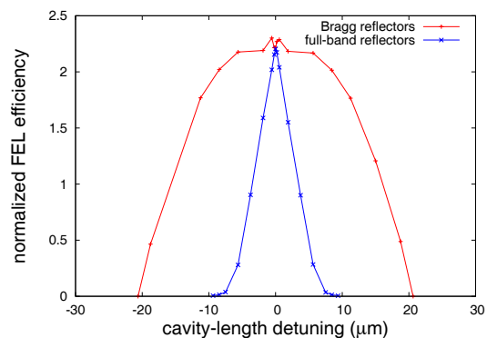
Figure 5: Cavity-length detuning curves for two types of reflectors.
