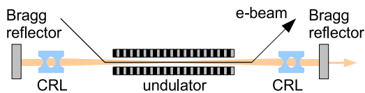
Figure 1: An XFEL oscillator with Bragg reflectors and compound refractive lenses (CRL) installed at a multi-GeV ERL.
