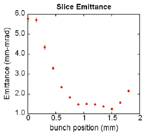
Figure 6: Slice emittance measurements. The slice length has been set to 150 \mu , i.e., about 0.5 ps.
