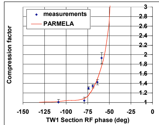
Figure 7: First test of velocity bunching: compression factor vs. the phase of the first TW section. Comparison between measurements and simulations
