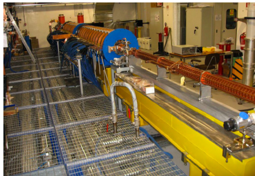
Figure 1 : Picture of the SPARC photoinjector showing the 3 accelerating structures with 2 long solenoids.
