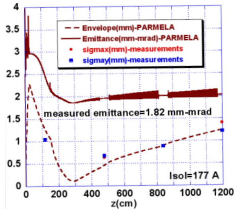
Figure 5 : PARMELA simulation of the envelope and emittance corresponding to the best measurement shown in Fig. 3 (Isol=177 A). The measured envelopes (blue rectangle) are also shown.
