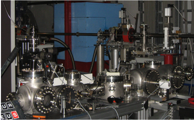
Figure 9 : Harmonic generation chamber in the SPARC Hall.
