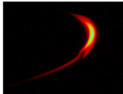
Figure 8 : Imaging of the longitudinal phase space on a screen downstream the dipole with the RF deflector on. Beam energy on the horizontal axis, beam phase on the vertical axis.
