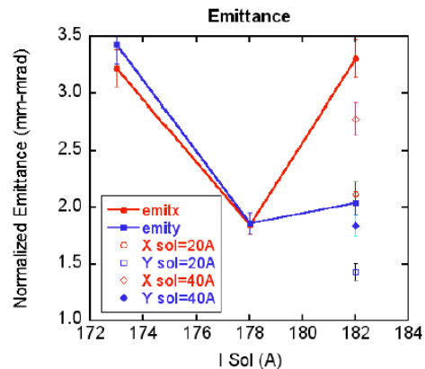
Figure 4 : Emittance measurement for different current settings of the gun solenoid and two values (20 A and 40 A) of the coils around the accelerating structures.
