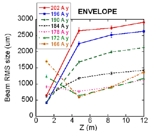
Figure 3 : Envelope measurements along the linac for different current settings of the Gun Solenoid. The bunch length was 6.5 ps, with 340 pC of charge and a rms size on the virtual cathode of about 340 \mu\text{m} .
