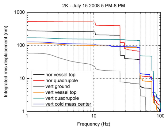
Figure 7: Typical rms amplitude spectra measured on Module 8 during its cold test on the CMTB.
