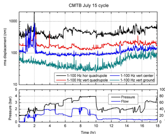
Figure 6: rms displacement integrated from 1 to 100 Hz measured on the cold mass for different settings of 4.5 K circuit, compared with the floor vibrations. In the first hour of the test the circuit was closed.
