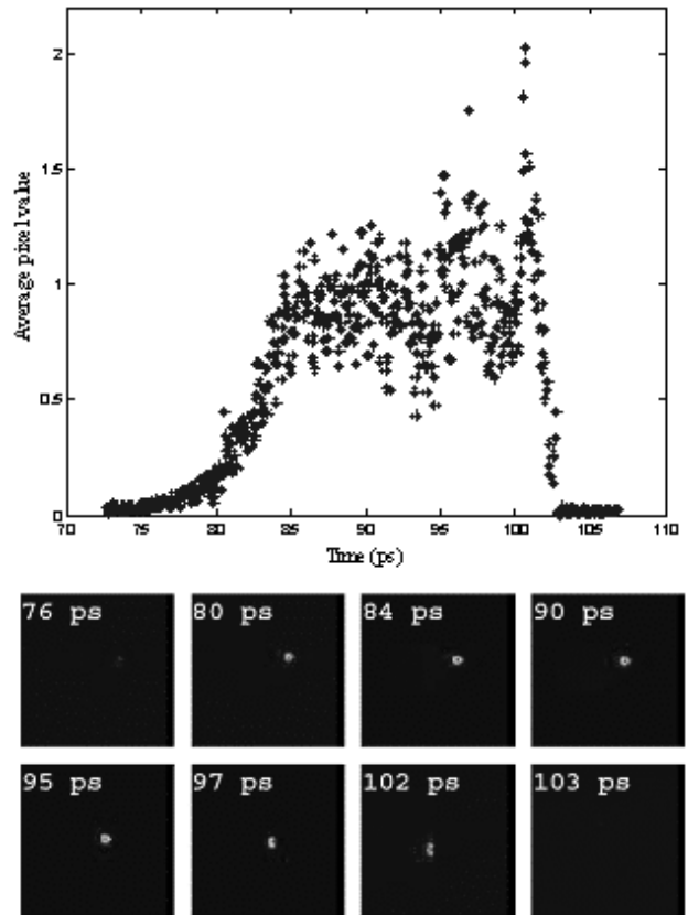
Figure 5: A sequence of pictures (bottom) recorded by a camera on OS2 as the 200 fs laser pulse samples different longitudinal slices of the electron bunch. The size of the area shown in the pictures is 5 mm by 5 mm. The upper plot shows the average pixel value in a small region around the spot. It shows a clear enhancement as the laser pulse passes the electron bunch from the tail of the bunch at the left, to the head of the bunch at the right.
