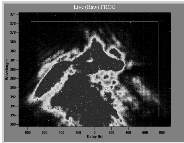
Figure 4: FROG trace illustrating the change of appearance of the trace when compressing the electron bunch over a certain limit.
