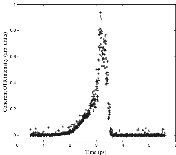
Figure 2: An example of a scan used to determine the position of the temporal overlap between the laser- and electron pulse. The enhancement of coherent OTR as a function of delay of the seed laser pulse reveals the overlap position.
