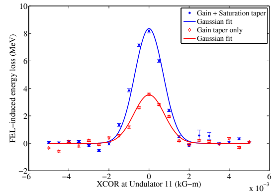
Figure 12: Measured FEL-induced electron energy loss as a function of dipole kick at undulator 11. The addition of a saturation taper can increase the FEL output by a factor of greater than 2.
