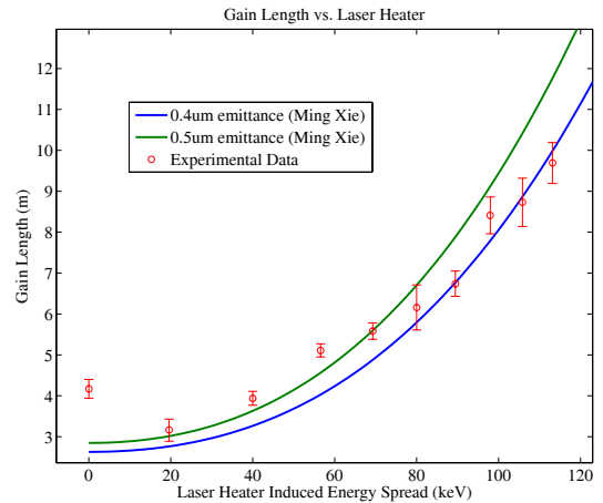
Figure 9: Gain length as a function of energy spread following the laser heater. Ming Xie scaling shown for 0.4, 0.5 \mu\text{m} emittances. We note the increased gain length with no laser heating (0 keV), hinting at the importance of the laser heater to suppress the microbunching instability. The nominal heater value induces a 20 keV energy spread.
