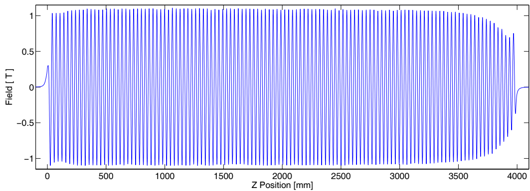
Figure 4: Field decay of up to 40% is observed at the edges of U33. This is a measurement with 9 mm gap size.
