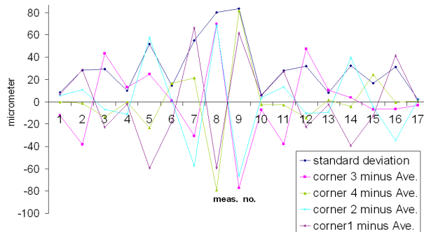
Figure 3: In several steps the gap size has been changed and the half gap displacement were measured with micrometer precision gauges. The average gap change is defined by the mean value of four measured displacements. The deviations in each corner with respect to the mean value is shown in the plot.
