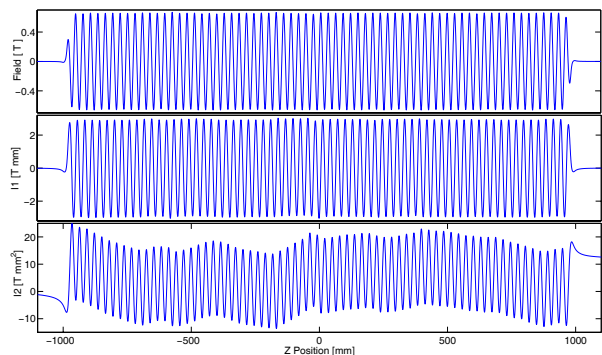
Figure 2: Preliminary Hall-probe measurements for U32 (12 mm gap) and corresponding field integrals.
