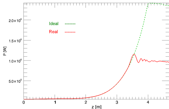
Figure 6: Simulated power gain curve for an HHG seed to the electron beam at the entrance of U33. For deteriorated field, the output power is affected by a factor of two with respect to the ideal case.
