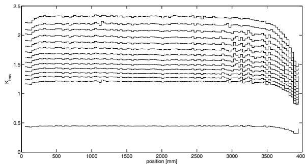
Figure 5: Measured B_y is used to plot variation of the undulator parameter K_{rms} along the device for different gaps. The top curve is for 9 mm gap size, the next curves are for larger gaps increasing in 0.5 mm steps up to 15 mm, the last one corresponds to 25 mm.
