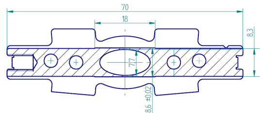
Figure 1: Cross-section of the undulator vacuum chamber
