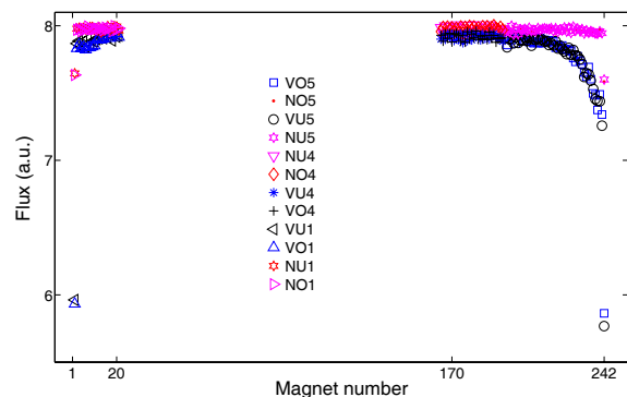
Figure 7: Comparison of the measured flux of magnets before re-magnetization (V) and after (N). Magnets in the upper jaw are marked with 'O' and in the lower jaw with 'U'. There are in total five modules and the entire magnets of upper and lower 5 th modules are re-magnetized. Some of the magnets in the modules 1 and 4 are also re-magnetized.
