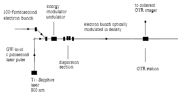
Figure 1: Schematic diagram of the coherent imager. The working principle is based on the optical modulation of the electron bunch and on emission of coherent OTR radiation from the metallic mirror.
