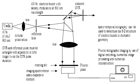
Figure 9: Multishot measurement of the 3D structure of electron bunches by use of spatio-temporal Fourier transform holography.
