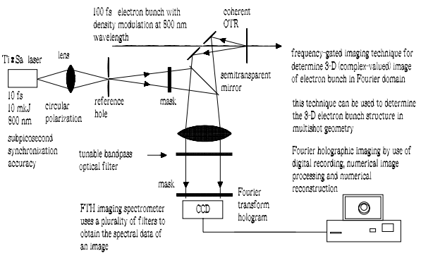
Figure 8: Multishot measurement of the 3D structure of electron bunches by use of frequency-gated Fourier transform holography.
