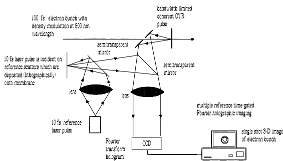
Figure 11: 3D electron bunch structure monitor by use of the HOTRI technique.
