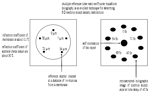
Figure 10: Membrane for time-resolved FTH with reference scatterers (left) and reconstructed holographic images of electron bunch slices (right).
