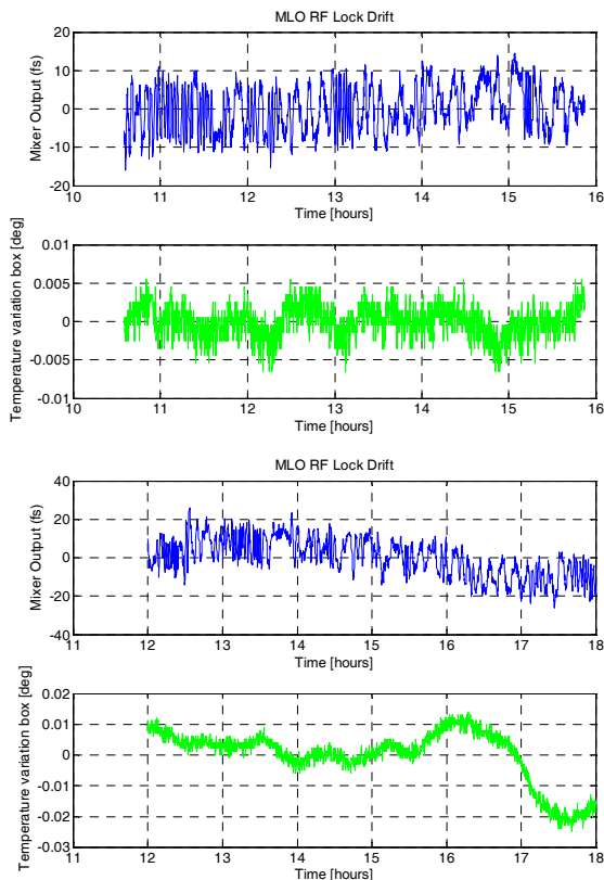
Figure 5: Drift of RF circuit with (top) and without (bottom) active temperature stabilization.
