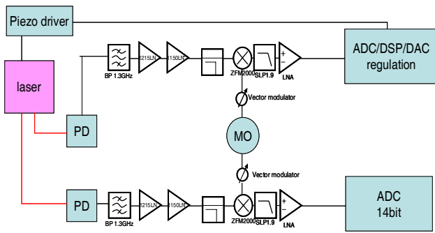
Figure 7: Out-of-loop setup. One photo-detector/down-mixer chain is used for the regulation and the other is used to measure the resulting phase stability.
