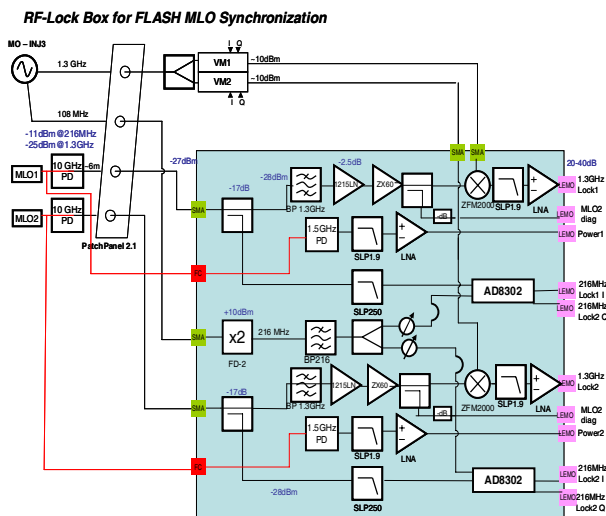
Figure 1: Schematic of MLO – MO phase measurements.
