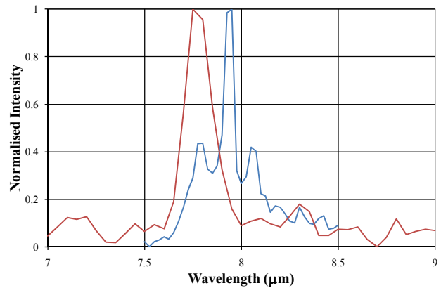
Figure 5: Two example spectra obtained during the commissioning that have very narrow bandwidth compared with the expected FWHM value of 3% (0.24 \mu\text{m} ).
