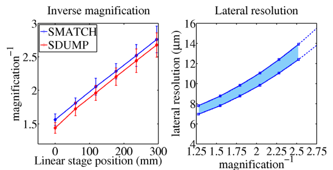
Figure 4: Performance of the camera optics at SDUMP and SMATCH. Left: Inverse magnification as function of the linear stage position (CCD camera + objective). Right: Lateral resolution as function of the inverse magnification.
