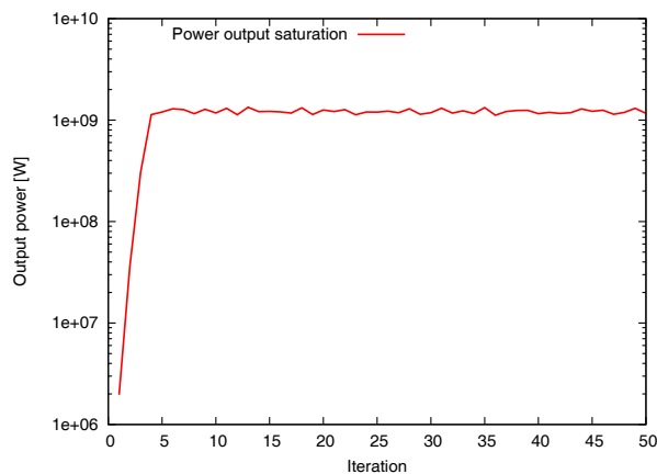
Figure 3: The evolution of the output power in the OFFELO. One iteration corresponds to one feed-back cycle of the system.
