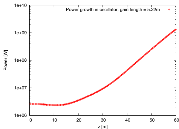
Figure 4: Power in main oscillator at 40th iteration.
