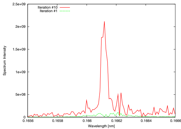
Figure 7: Evolution of the OFFELO spectrum during first ten iterations.
