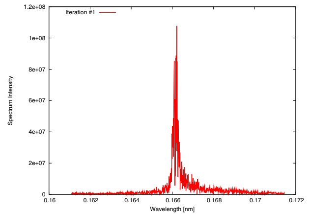
Figure 5: Spectrum of the radiation at the pass #1.
