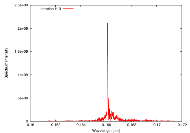
Figure 6: Spectrum of the radiation at the pass #10.
