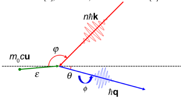
Figure 2: Interaction geometry.
