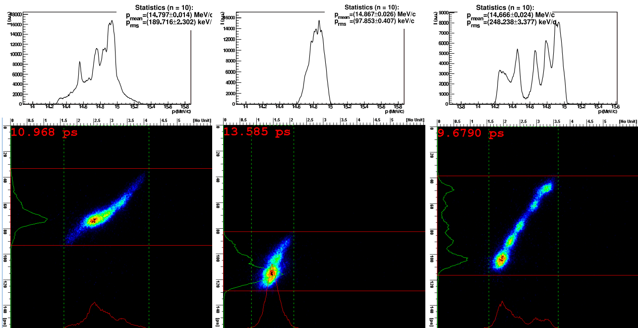
Figure 5: The streak camera image of the electron bunch (bottom) with introducing 16.88% modulation on the laser temporal profile, compared to the results from MAMA (top) for the maximum booster RF launch phase plus 10° (right), the maximum phase (middle) and maximum phase minus 10° (left).
