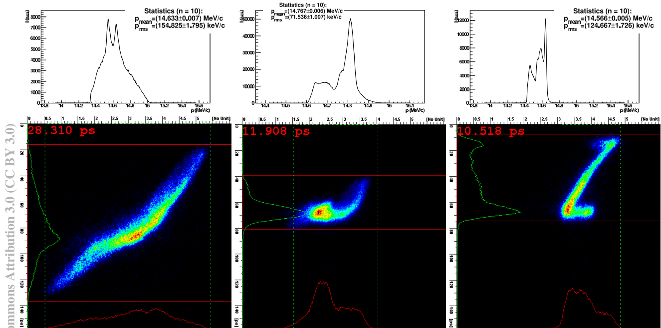
Figure 2: The streak camera image of the electron bunch (bottom) compared to the results from MAMA (top) for the maximum booster RF launch phase plus 10° (right), the maximum phase (middle) and maximum phase minus 10° (left). The temporal distribution of the streak image is flipped due to the momentum compaction factor of the deflecting dipole magnet.
