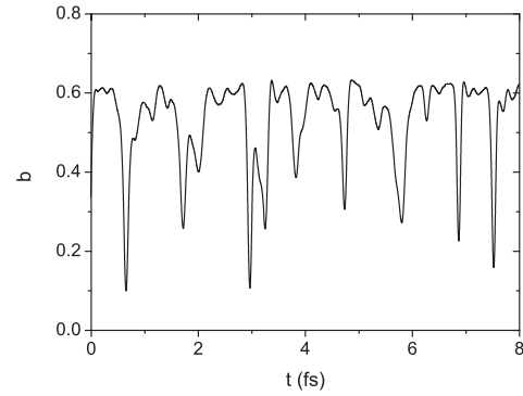
Figure 5: Modulus of bunching factor versus time at the exit of the planar undulator SASE3 (position 55 m on Fig. 4). A central part of the electron bunch is shown.
