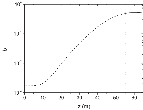
Figure 4: Evolution of the ensemble averaged rms bunching factor along the planar undulator SASE3 (dash) and the helical afterburner (solid).
