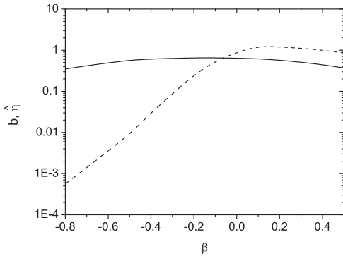
Figure 2: Ensemble averaged rms bunching factor (solid) and normalized FEL efficiency (dash) at saturation point (position with maximum bunching factor) versus taper strength parameter. Energy spread parameter is \hat{\Lambda}_T = 0.2 .
