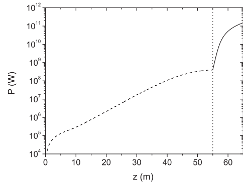
Figure 6: FEL power versus the length of the planar main undulator SASE3 (dash) and the helical afterburner (solid).
