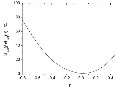
Figure 3: Relative increase of the saturation length (defined as a length of the undulator at which maximum bunching is achieved) versus taper strength parameter. Energy spread parameter is \hat{\Lambda}_T = 0.2 .
