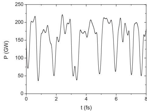
Figure 7: Peak power of circularly polarized radiation at the exit of the afterburner (position 65 m on Fig. 6). A central part of the X-ray pulse is shown.
