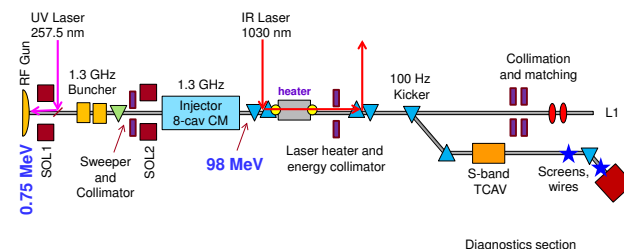
Figure 1: Injector layout.
