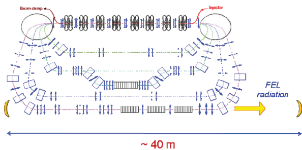
Figure 5: The third stage ERL with FEL undulators and optical cavity.
