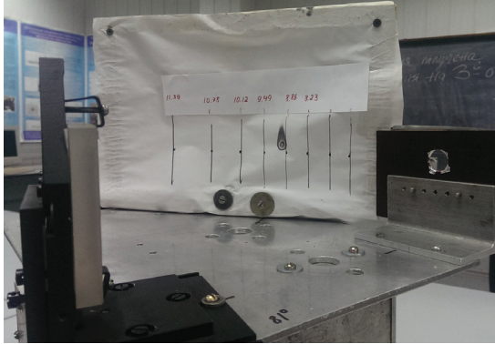
Figure 9: Radiation wavelength measurement experiment.
