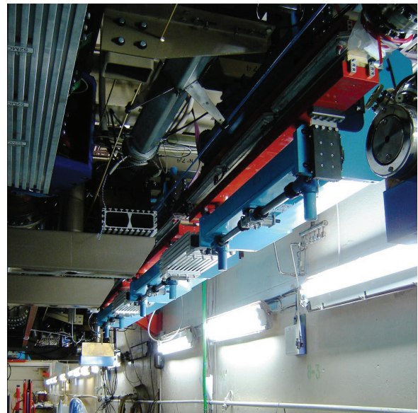
Figure 6: The third stage FEL undulator sections.
