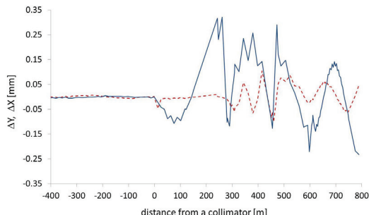
Figure 3: The vertical (solid line) and horizontal (dotted line) projections of the beam trajectory, where the bottom jaw of a vertical collimator is moved close to the beam.
