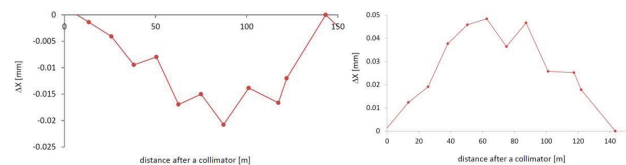
Figure 2: Difference of the horizontal projections of the measured and reference beam trajectories downstream of a horizontal collimator when the left or right jaw moved towards the beam.
