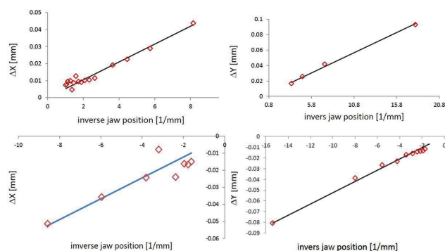
Figure 5: Comparison of the measured beam displacement after a collimator (red diamonds) with the theoretical prediction (black solid line) for four jaws of the horizontal and vertical collimators.
