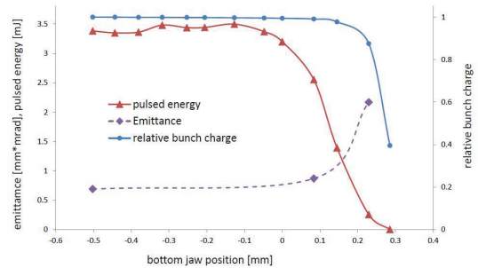
Figure 7: The FEL pulse energy (triangles), the beam emittance (diamonds) and the relative bunch charge (circles) versus the collimator jaw position.
