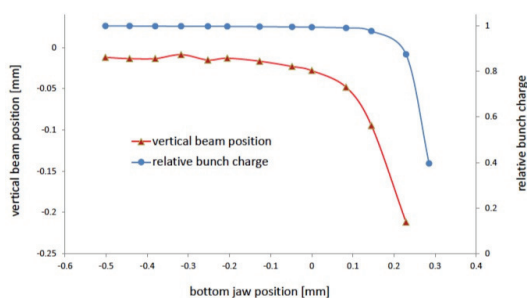
Figure 4: A vertical beam position (the line with triangles) and a relative bunch charge (line with circles) versus position of the collimator bottom jaw.
