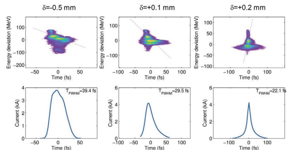
Figure 8: Bunch images on the phase plane for different positions of the collimator jaw.
