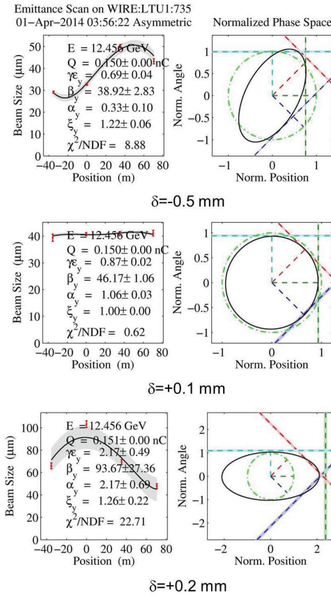
Figure 6: Emittance measurements for different positions of the collimator jaw: -0.5, +0.1, +0.2 mm.
