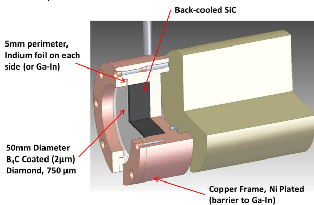
Figure 8: A 3D rendering of the CVD stopper (active burn-through monitor not shown).
