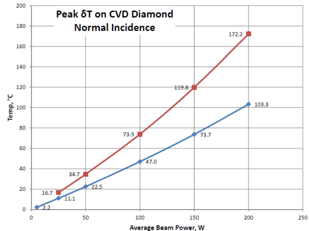
Figure 3: The steady state maximum temperature in the diamond for the 1.3 keV SXR (blue line) and 5 keV HXR (red line) cases as a function of the (CW) incident power for the geometry shown in Figure 2.
