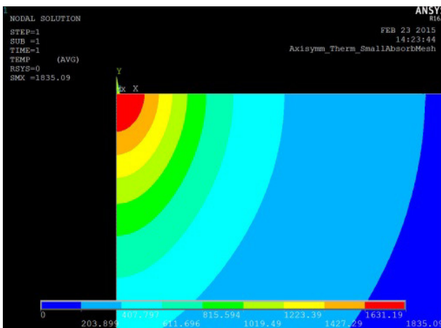
Figure 11: Temperature distribution in B 4 C under normal incidence.
