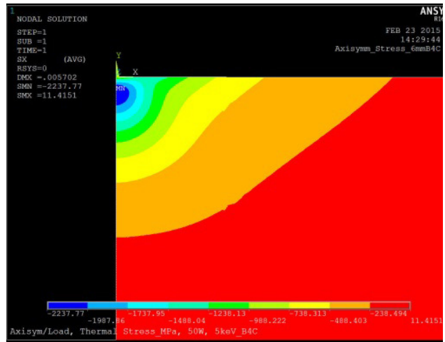
Figure 12: Radial Stress distribution in B 4 C under normal incidence.
