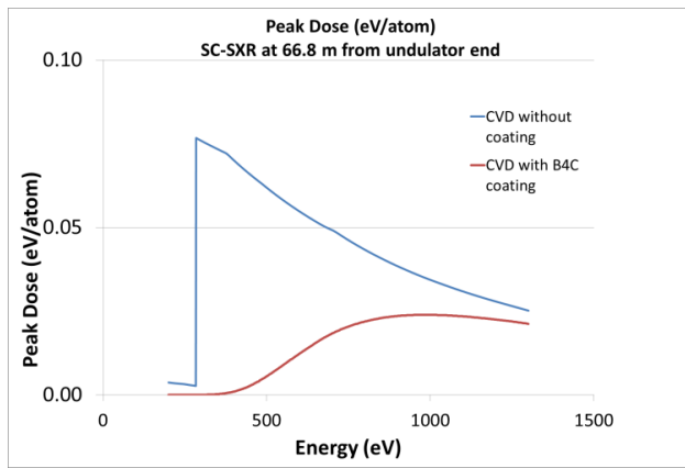
Figure 7: The peak dose of coated (red line) and uncoated CVD diamond (blue line).
