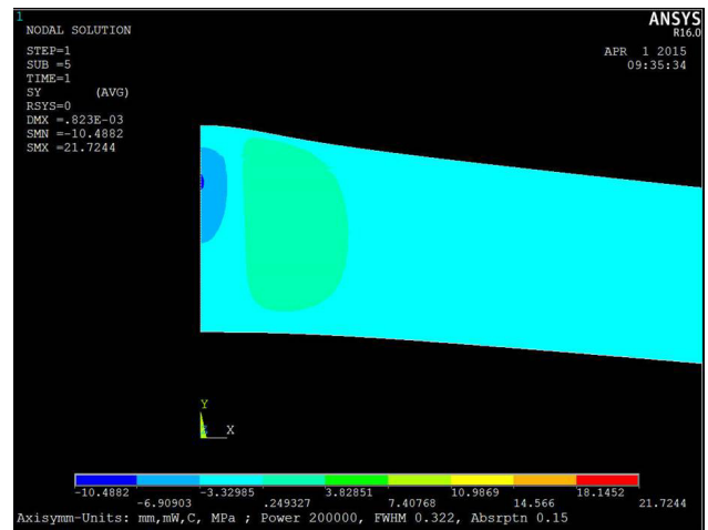
Figure 6: Axial stresses. Extreme values: 7.4 MPa (tensile), -10.5 MPa (compressive).
