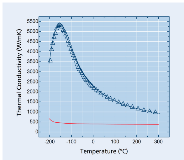
Figure 1: The thermal conductivity of CVD diamond (blue line) and copper (red line) for comparison [data taken from Diamond Materials GmbH].
