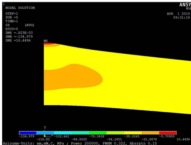
Figure 5: Radial stresses. Extreme values: 10.45 MPa (tensile), -38 MPa (compressive).
