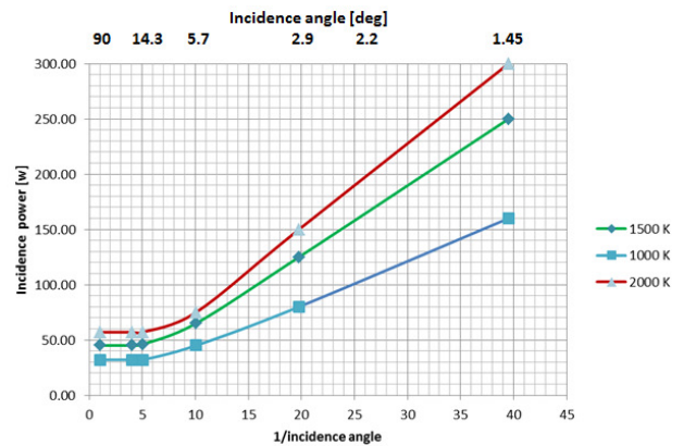
Figure 13: Dependence between the angle of incidence and the incident power for constant surface temperature.
