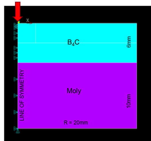
Figure 9: The geometry and boundary conditions of the B 4 C stopper model at normal incidence.
