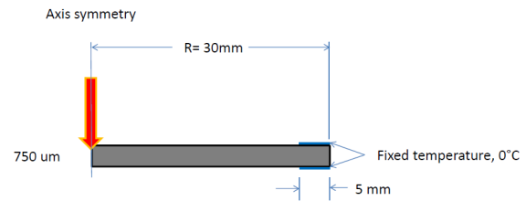
Figure 2: The schematic of a perimeter cooled CVD diamond used in simulations. The FEL beam is incident normal to the top surface and at the center of a 750 \mu\text{m} thick diamond disk of 30 mm in radius with the edge being held to a fixed temperature of 0°C.
