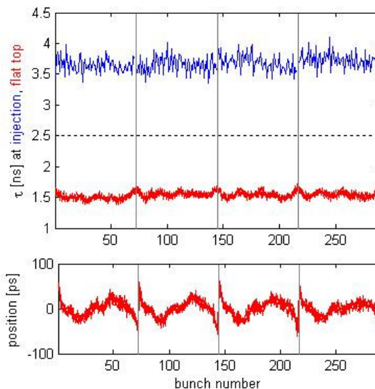
Figure 2: The bunch length ( 4\sigma Gaussian fit) along the 4 LHC batches for nominal intensity at injection (top, blue curve) and extraction (bottom, red curve) from the SPS - top figure. Bunch position over four LHC batches at extraction from the SPS - bottom figure.
