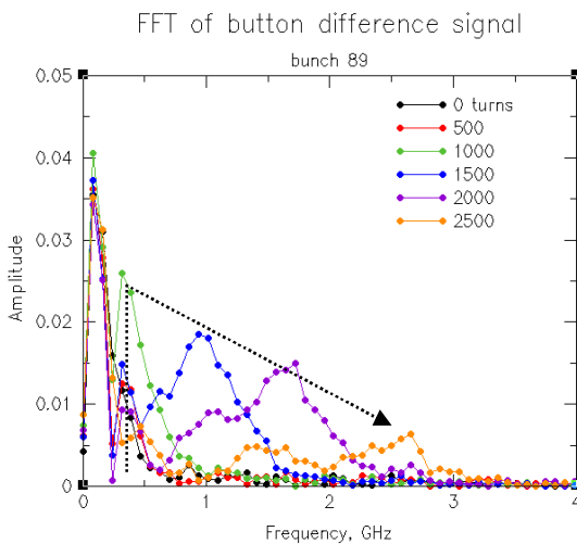
Figure 7: The evolution of the transverse instability spectrum with the time. The traces are taken with 6.4 ms interval.
