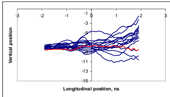
Figure 6: The transverse instability development. The traces are taken with 4ms interval. The head of the bunch is on the left side of the plot. The vertical axis shows the vertical position in arbitrary units.
