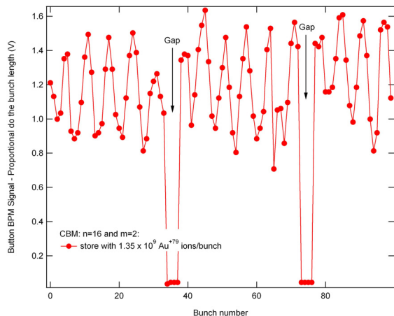
Figure 3: The signal proportional to bunch length is shown at some short time after the transition for all bunches of the beam. The oscillation phase varies with the bunch position in the train. The bunch pattern had two small gaps.
