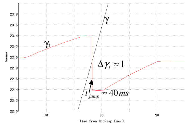
Figure 1: The schematic of \gamma_t and \gamma changes trough the transition region with 40 ms long \gamma_t -jump.
