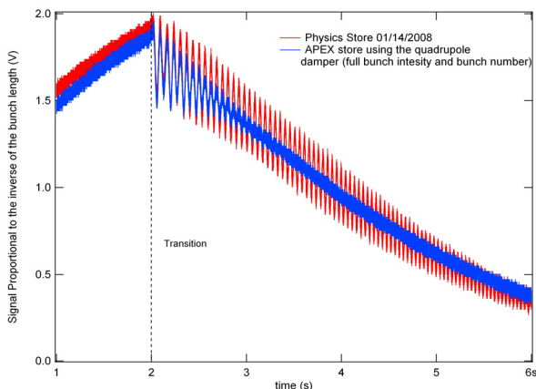
Figure 2: The comparison of the bunch length oscillations after the transition with the feedback on and off. Plotted signal is proportional to the inverse of the bunch length.
