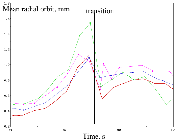
Figure 4: The Yellow mean radial orbit through the transition area on several consecutive ramps.
