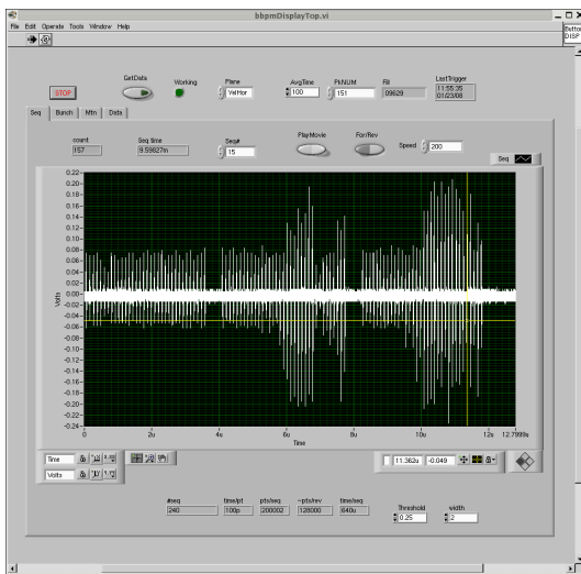
Figure 5: The instability, as measured by a button BPM, affects bunches at the end of the mini-trains.
