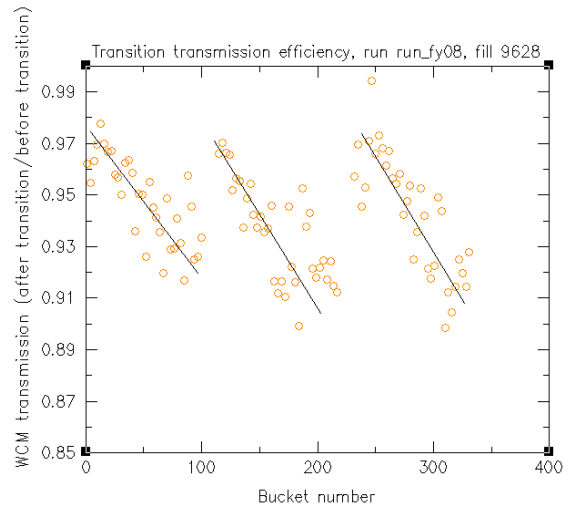
Figure 6: The efficiency of bunch intensity transmission through the transition area versus bunch position in the train. The bunch pattern shown contains two mini-gaps.
