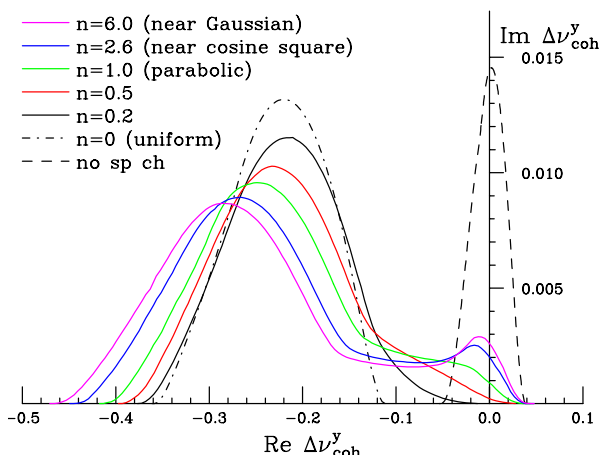
Figure 6: (Color) Stability contours for various longitudinal generalized elliptical bunch distributions, from n = 0 , the uniform distribution, to n = 1/2 , the elliptical distribution, to n = 1 , the parabolic distribution, to n = 2.6 , roughly the cosine square distribution, and to n = 6 , roughly the Gaussian distribution. It is clear that as n increases the stability contour spreads out and more reaching and eventually covering \text{Re } \Delta\nu_{\text{coh}}^y = 0 , thus providing Landau damping if |\text{Re } Z_1^\perp| is not too large. The stability contour for octupole alone without space-charge is also shown in dashes.
