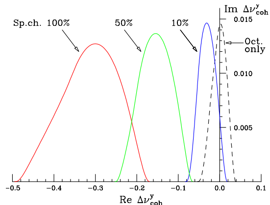
Figure 1: Stability contour from octupole alone shown in dashes changes to the red curve with the introduction of full space-charge force. It changes to the green and blue curves when space-charge is reduced to, respectively, 50% and 10%.
