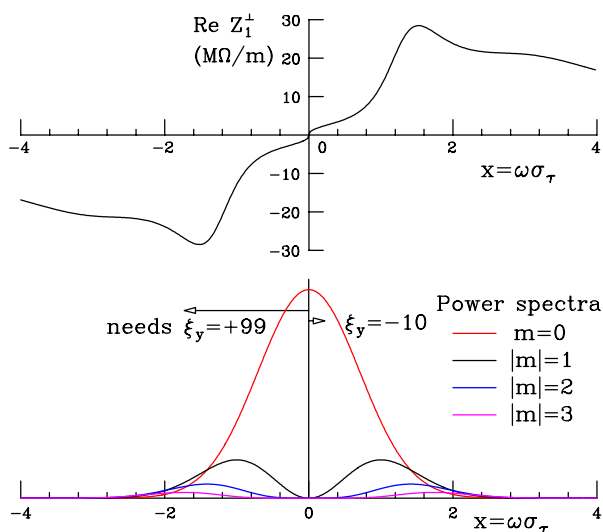
Figure 9: Plot showing shifts of power spectra of azimuthal modes under chromaticity \xi_y along the frequency axis with respect to the transverse impedance \text{Re } Z_1^+ .
