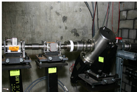
Figure 1: Pre-target beam instrumentation station, showing horizontal and vertical BPM's and SEM profile monitor.
