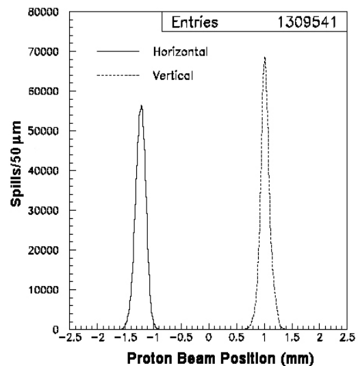
Figure 2: Histogram of proton beam position as seen by target BPM's for both horizontal and vertical planes. Beam is centered on the target, which is located at (x,y)=(-1.2,+1.0\text{mm}) .
