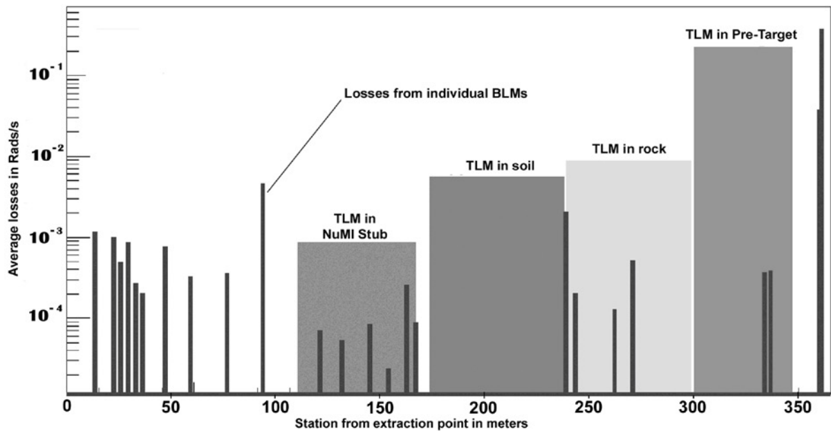
Figure 3. Beam loss along the NuMI proton line averaging for all beam extractions over a one month period. The beam loss scale can be obtained by the reading of the most downstream BLM which sees beam loss from the target profile monitor. This monitor scatters 10^{-5} of the beam passing through it.
