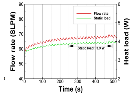
Figure 6: Measurement of static thermal load of quarter wave resonator cryomodule.
