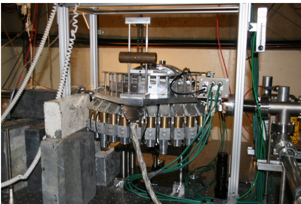
Figure 3: The E-203 experimental apparatus installed on the FACET beam line and showing the array of pyroelectric detectors used to detect the signal.
