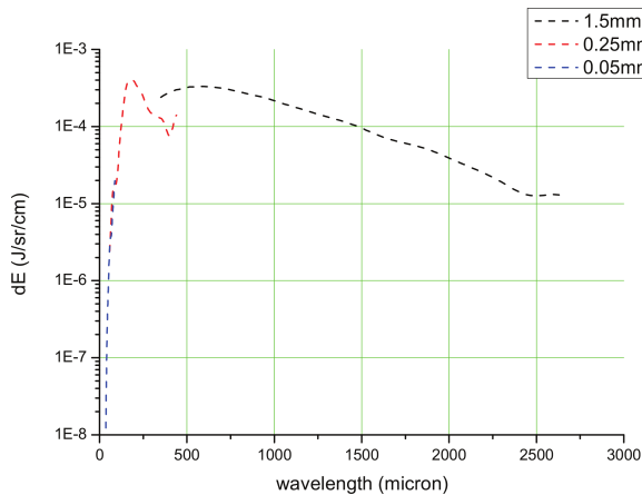
Figure 6: The expected Coherent Smith-Purcell radiation spectrum in a “notch collimator” configuration. Each color correspond to a different grating.
