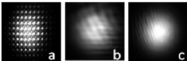
Figure 8: (a) Wavelength diffraction pattern with mirrors in floating state; (b) Distorted beam image; (c) Undistorted image with all pixels set at +12^\circ .
