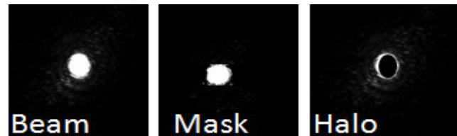
Figure 6: Illustration of adaptive masking technique for an arbitrary beam profile.
