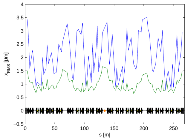
Figure 3: Horizontal RMS beam displacement.
