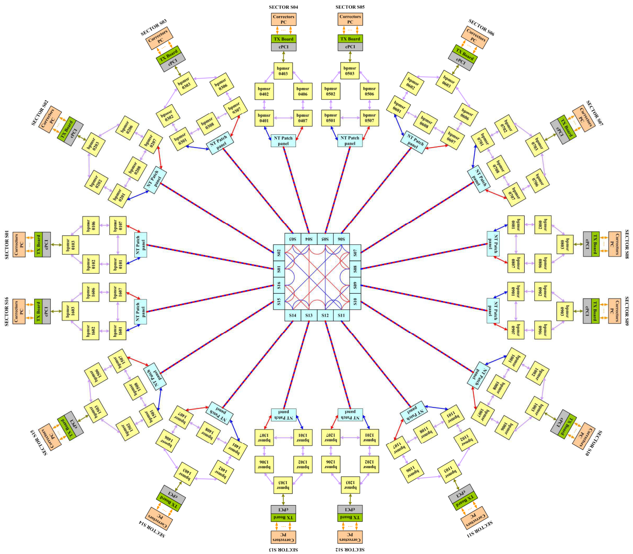
Figure 1: ALBA FOFB topology. Shown elements are: Libera Brilliance eBPM electronics ( bpmstr XXXX, depending on SR sector and unit), FOFB processing node ( cPCI ), data transition board ( TX Board ), corrector magnets power converters ( Correctors PC ), optical patch panels on Network racks ( NT Patch panel ) and the main interconnection panel in the center.
