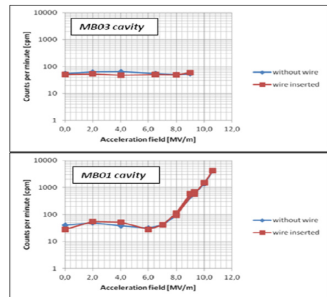
Figure 7: value of count rate emitted from cryomodule and detected by BEM.
