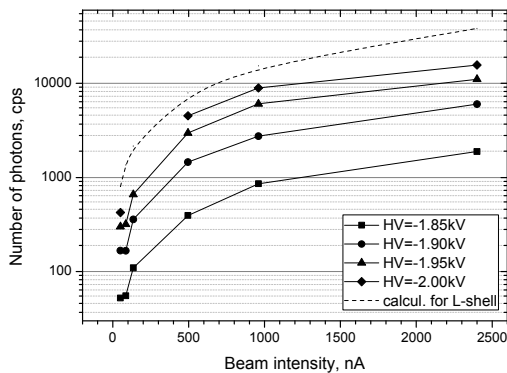
Figure 5: Comparison of count rates for different values intensities and applied voltage. Theoretical estimation of count rate due L-shell ionisation is presented.
