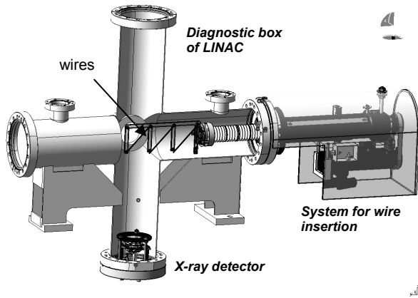
Figure 2: General view of BEM installed at diagnostic box of LINAC.
