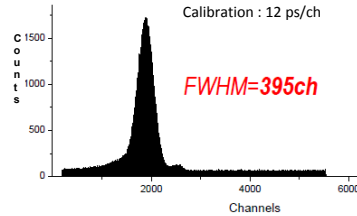
Figure 3: Measured bunch profile of 36 Ar +18 with 2.4 μA beam intensity (Value of MCP applied voltage of 1.95kV and time acquisition =60 s).
