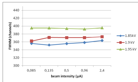
Figure 4: Measured FWHM bunch of 36 Ar +18 versus beam intensity.
