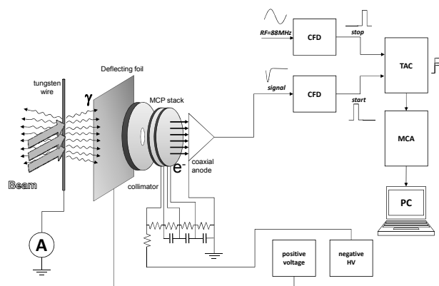
Figure 1: Principal schema of operation of BEM electronics.
