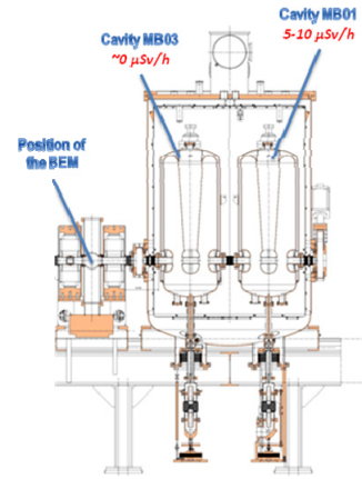
Figure 6: Installation of BEM set close to cryomodule B.
