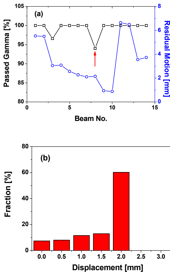
Figure 7: (a) The percentages of passed gamma and residual motion for fourteen irradiations. (b) Probability density functions of the displacement during the gate of the 8th irradiation indicated by arrows in (a).
