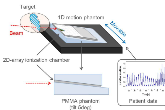
Figure 2: Schematic view of measurement setup for the additional patient-specific QA.
