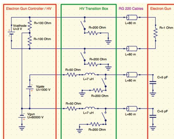
Figure 17: Schematic of HV connections to the electron gun.
