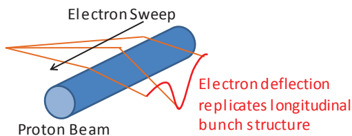
Figure 3: Deflection when the electron beam is scanned along the direction of the proton bunch with duration similar to the bunch structure.
