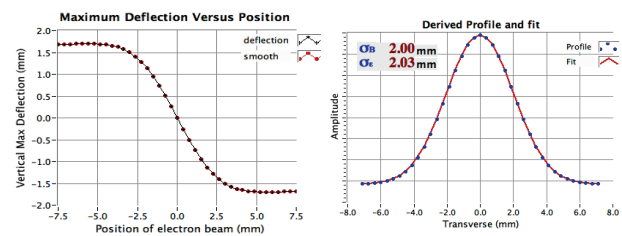
Figure 10: Deflection plot of pencil electron beam, and the derivative of it, showing agreement to better than 2%.
