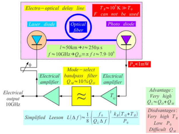
Figure 13: Opto-electronic oscillator.
