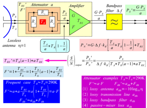
Figure 6: Attenuator noise.
