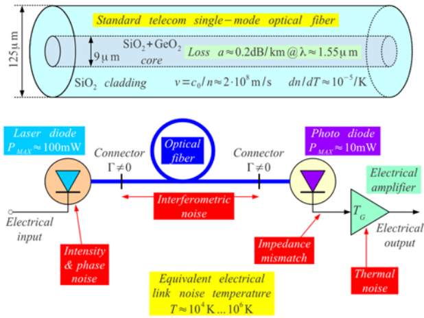
Figure 12: Optical-fiber link.
