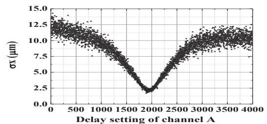
Figure 5: Measurement precision for changing the delay settings of channel A.
