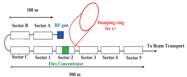
Figure 1: Schematics drawing of SuperKEKB injector linac. The coloured parts will be newly installed for SuperKEKB project.
