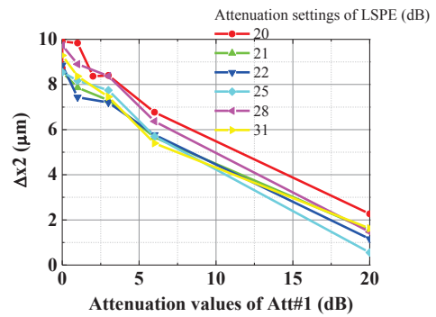
Figure 9: Variation of second bunch measurement accuracy by changing the attenuator setting of first bunch simulated signal.
