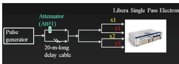
Figure 8: Experimental setup for evaluating the simulated second bunch beam position accuracy.
