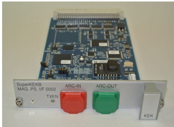
Figure 2: The upgraded PSICM (Power Supply Interface Controller Module), used for the magnet power supply control, for SuperKEKB.
