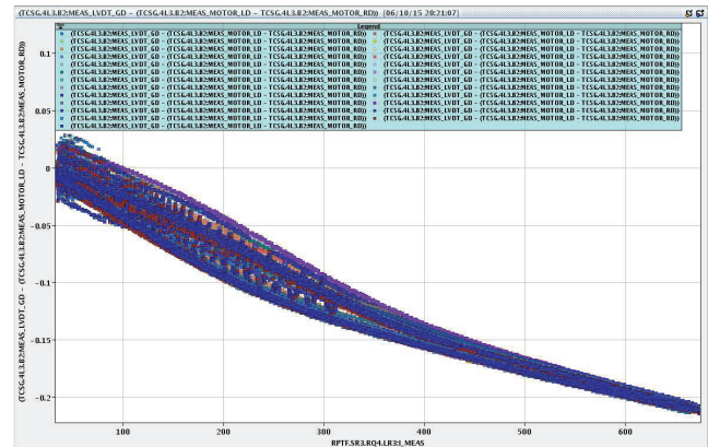
Figure 6: Correlation of the collimator jaw gap motor-LVDT offset and the current in a nearby magnet.
