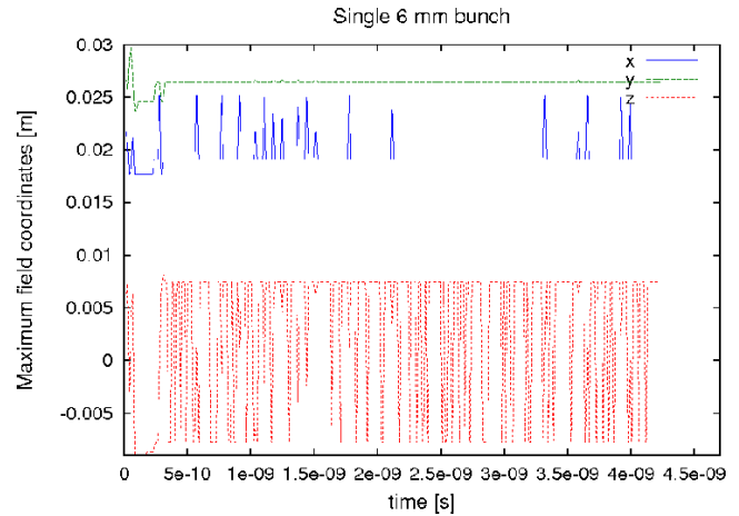
Figure 8: Coordinates of the maximum electric field strength in the vicinity of the BPM. z = 0 is the position of the BPM along the z -axis beam direction. The maximum field position oscillates between the upbeam and downbeam parts of the button.
